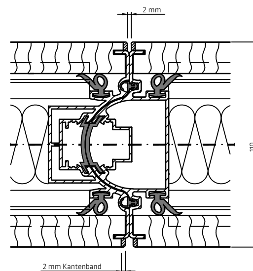
Elementkoppeling 110 K/A
