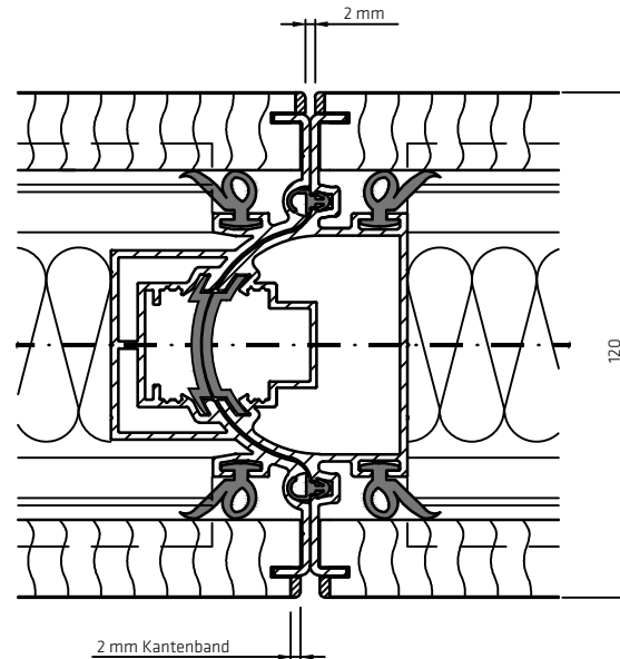
Elementkoppeling 120 K/A
