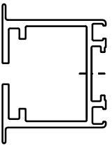
MR-S Rail
