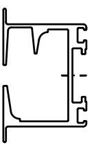
MR-1 Rail
